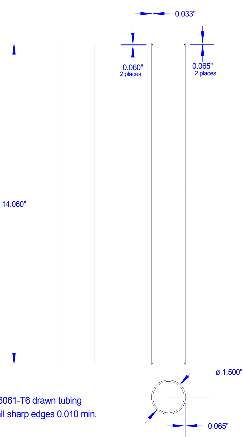
Impulser-X Rocket Motor Casing
