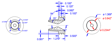
Nozzle assembly
