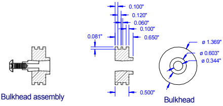
Bulkhead
