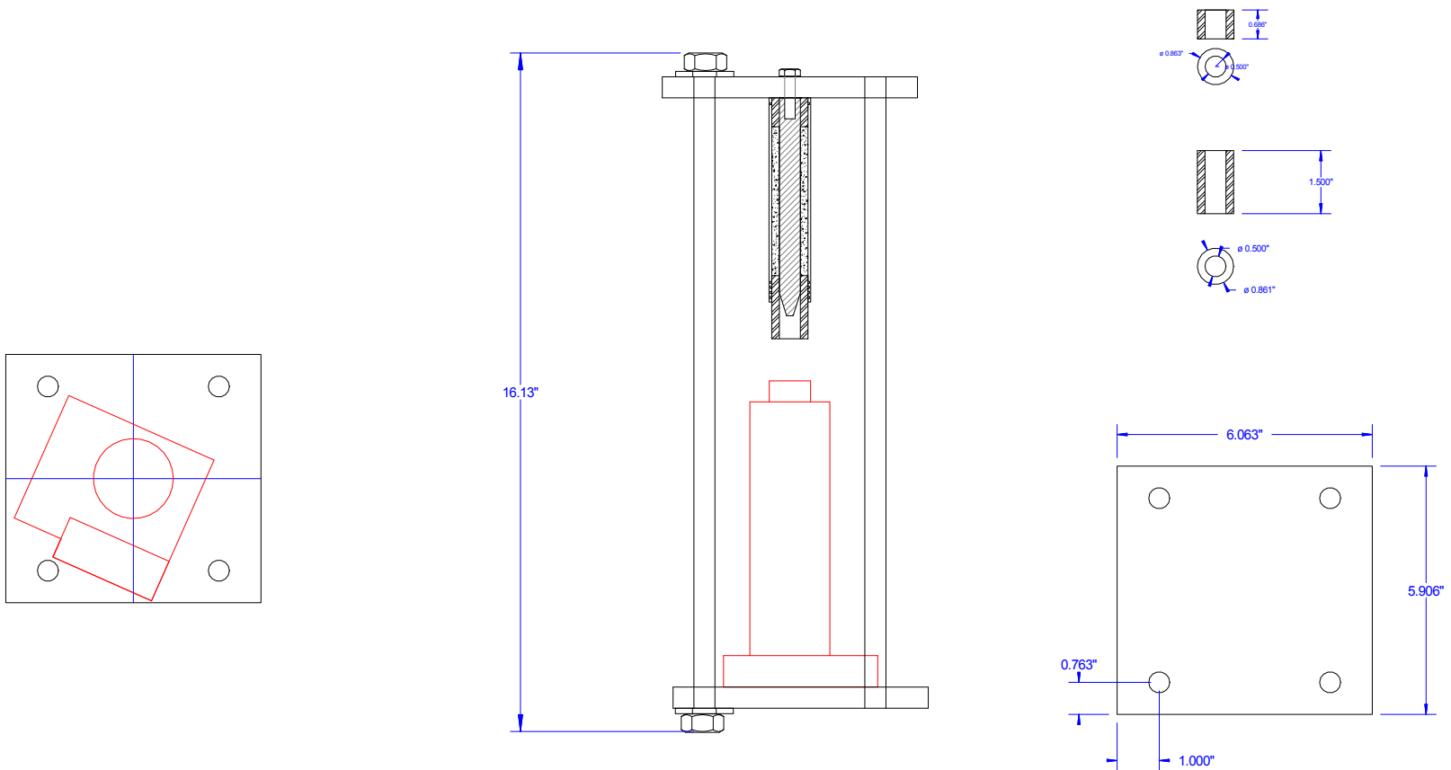
Compression mould for AN-Al experimental propellants
