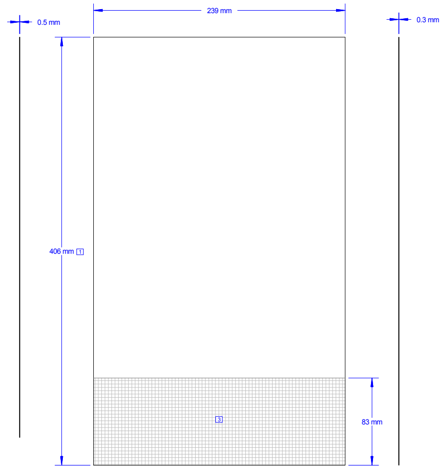
Rod-grain spacer (flat development)
