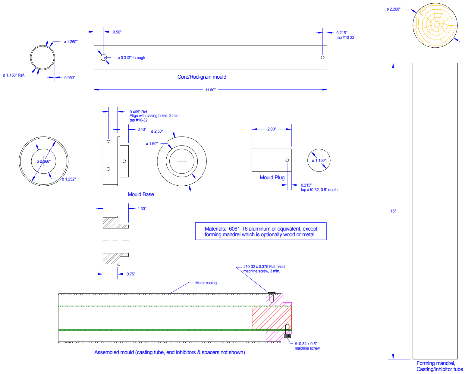
Paradigm Rocket Motor propellant casting mould assembly
