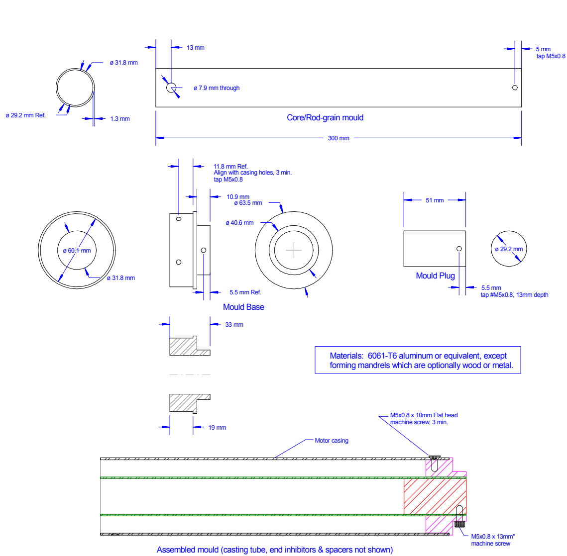
Paradigm Rocket Motor propellant casting mould assembly
