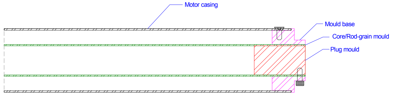
Assembled mould (casting tube, end inhibitors & spacers not shown)
