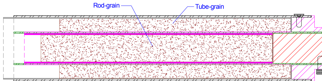
Assembled mould with packed propellant.
